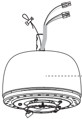
5.Motor Assembly
