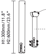
3.Downrod
