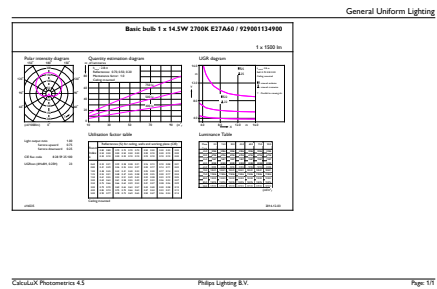
LEDbulb, Bulb A19 14.5W-100W 2700K 1500lm
