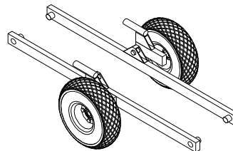
Side supports with wheel assemblies
