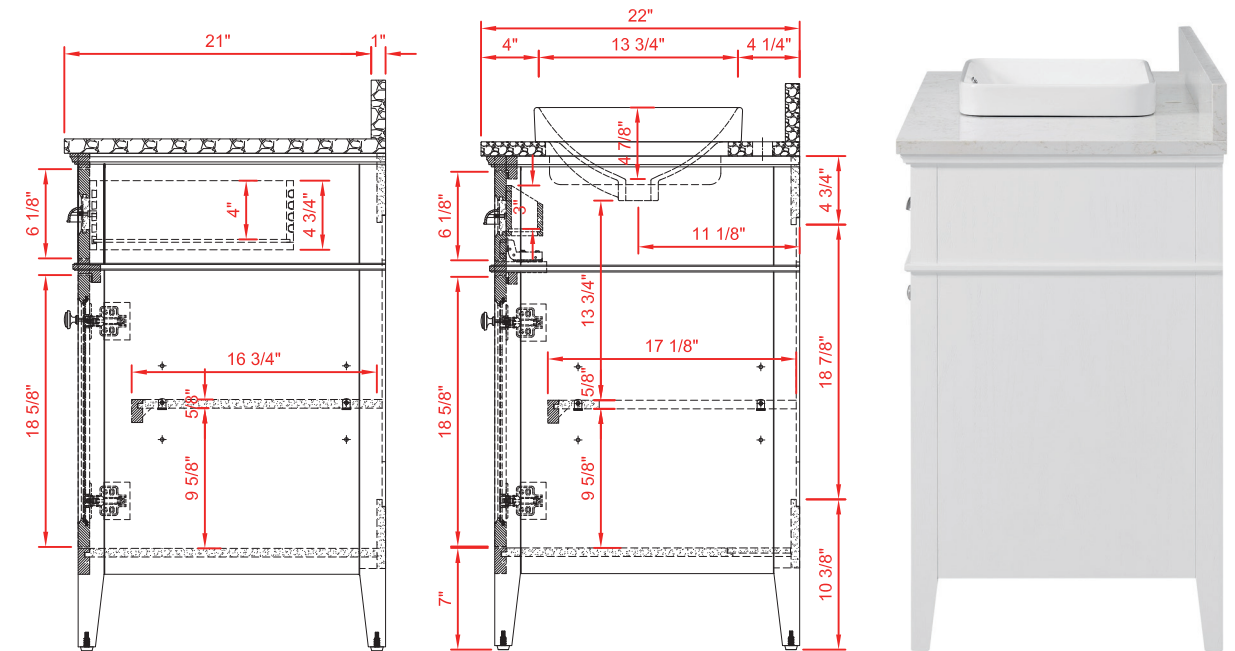
SIDE VIEW
