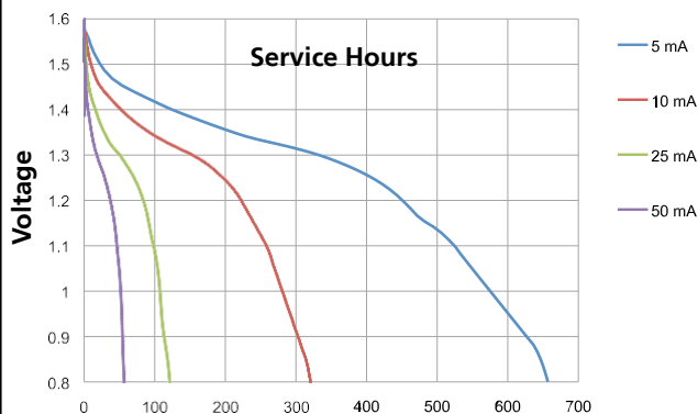
Procell AA Constant Current
