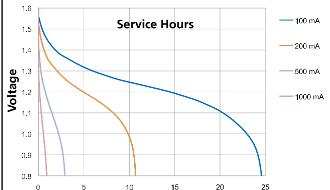
Procell AA Constant Current
