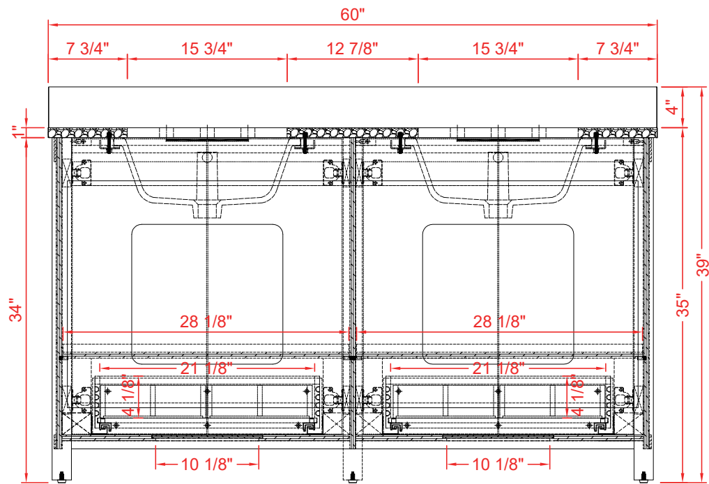
BACK VIEW
