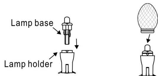
Fig.2 Replace with the spare lamp
