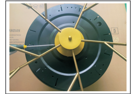
Step 5. Install and fix the lamp body on the chassis with screws.
