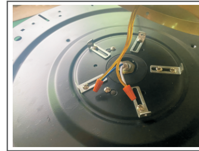
Step 4. Connect the power cable.
