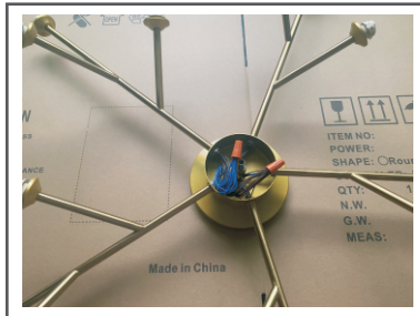
Step 1. Fix the light arm to the fan light body with a tool.
