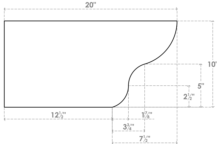
SIDE PROFILE
