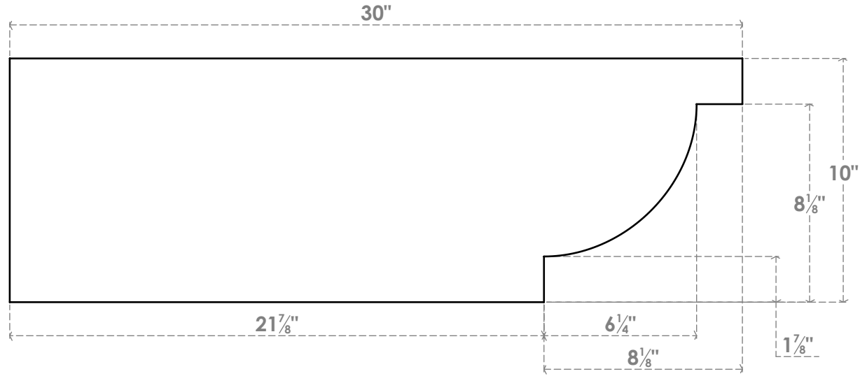
SIDE PROFILE
