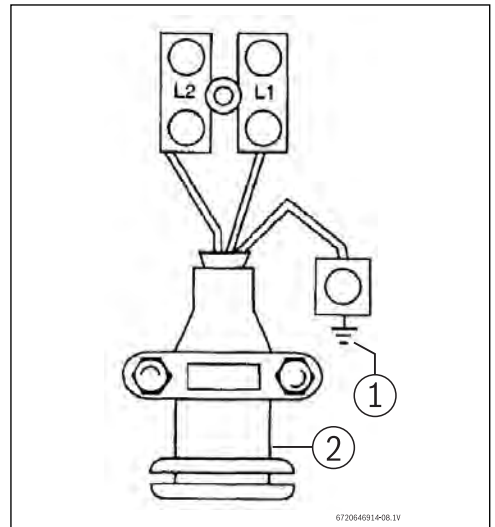
Fig. 4 Cable termination
