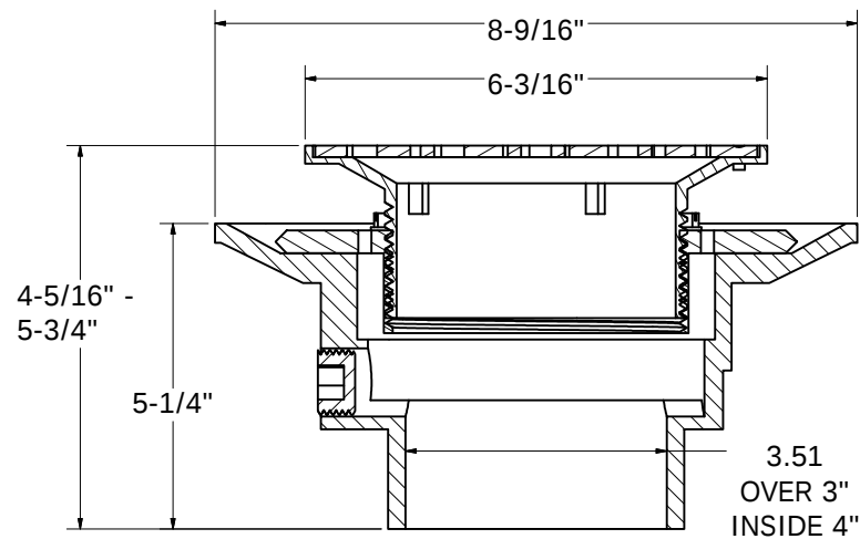
SECTION A-A SCALE .7
