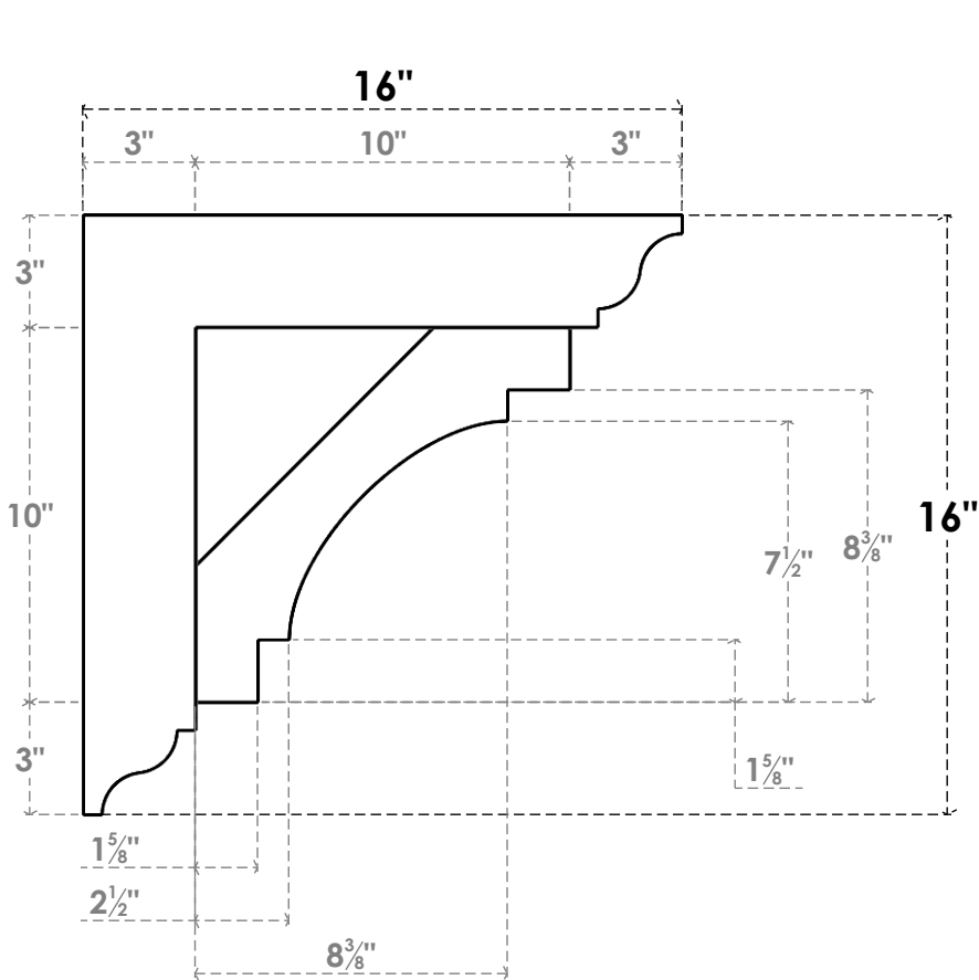
SIDE PROFILE
