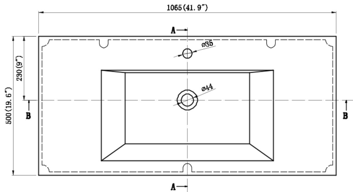
SECTION B-B
