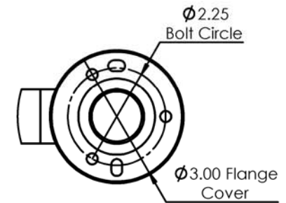
Flange Detail A
