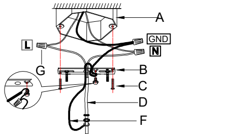
Wire Connection Diagram:
