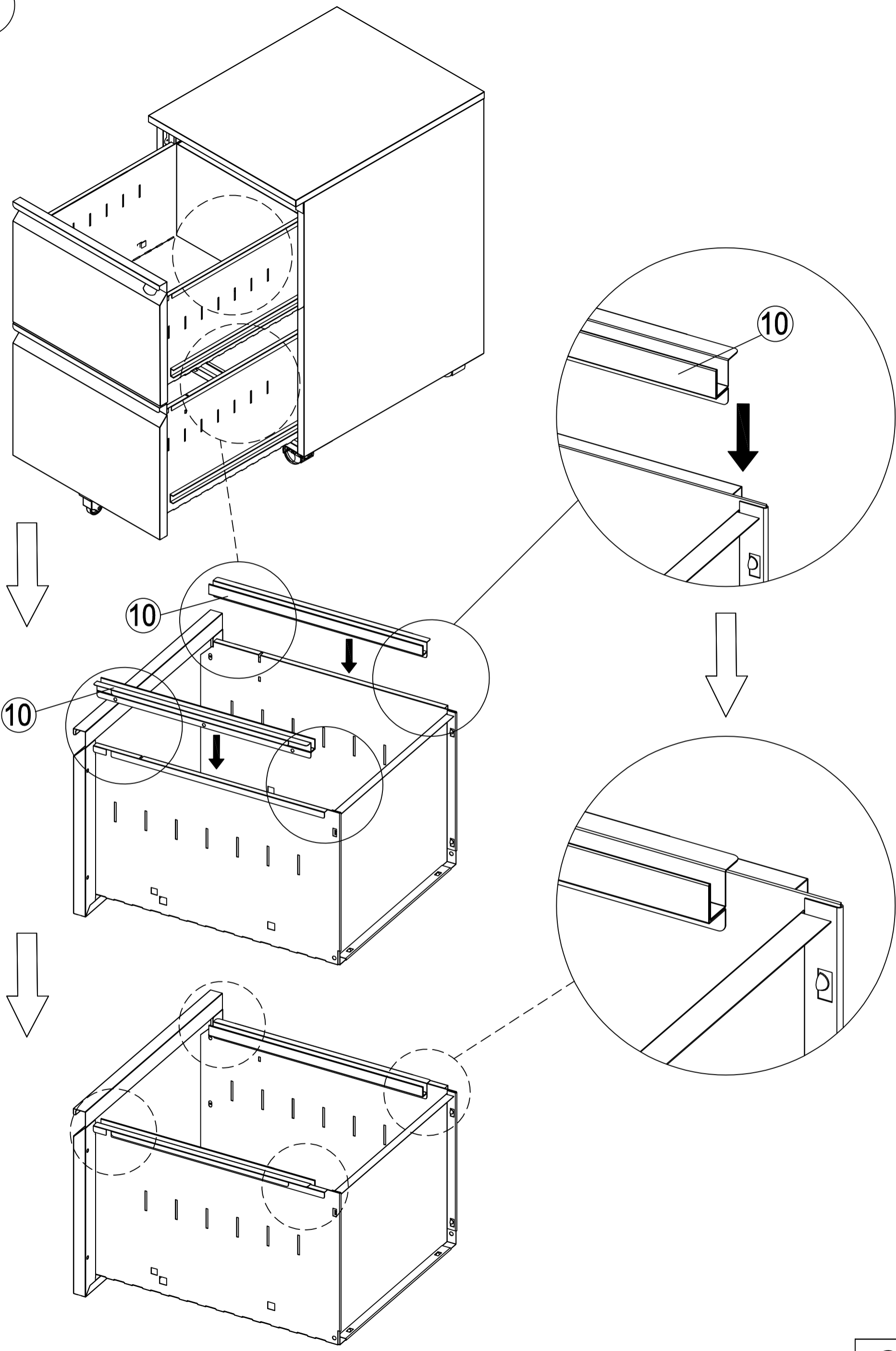
17. Assemble 10 on both drawers.
