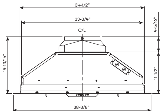
AK8200BS & AK8300BSX Side
