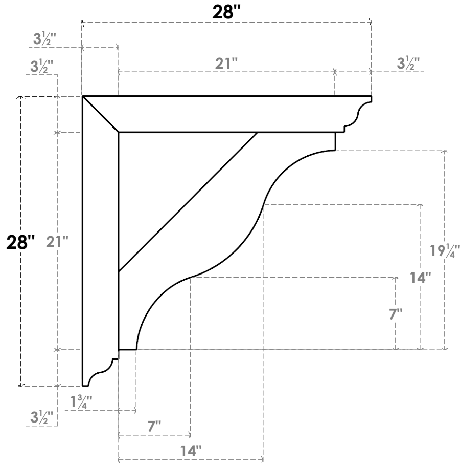
SIDE PROFILE
