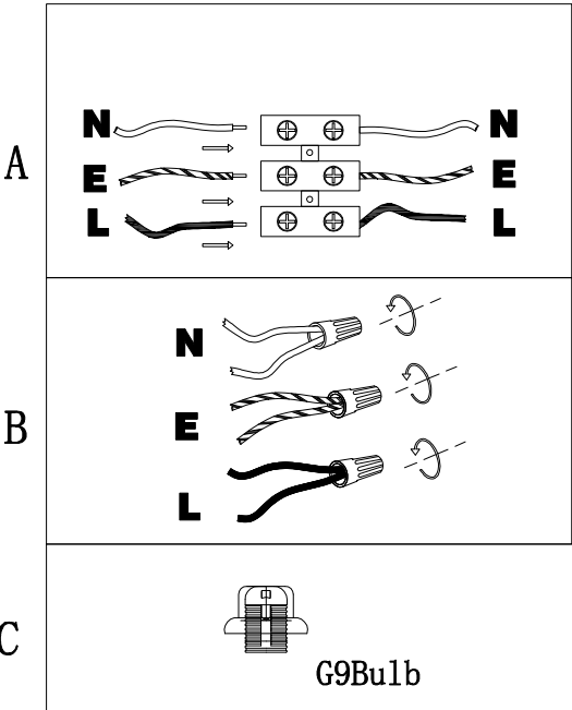
Wiring diagram
