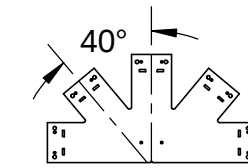
56620 10:12 Truss Base Fan (TBF-10-12)
