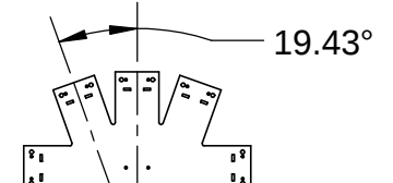
56642 4:12 Truss Base Fan (TBF-4-12)
