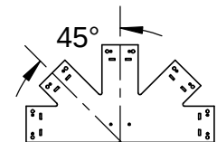
56644 12:12 Truss Base Fan (TBF-12-12)
