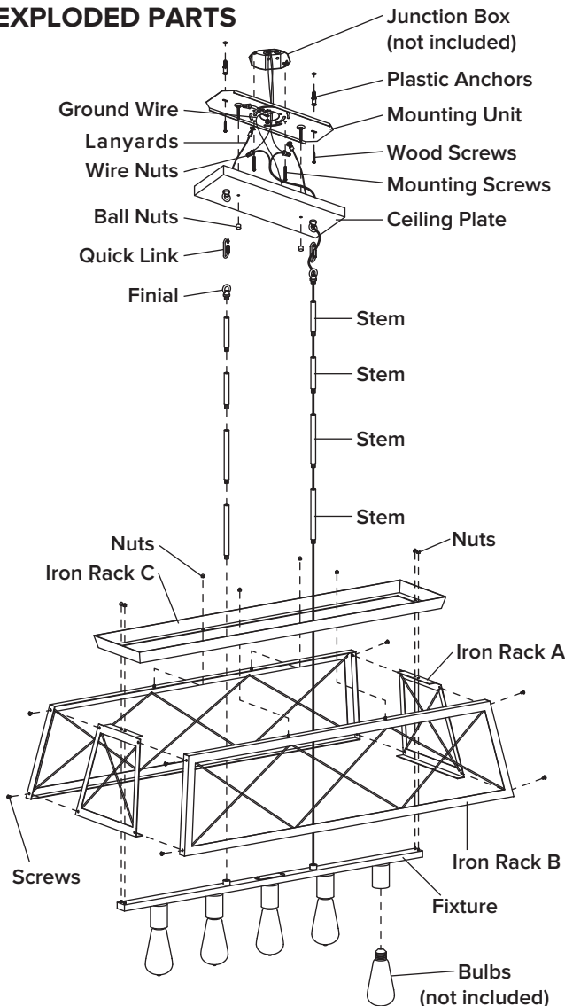
Fixture
