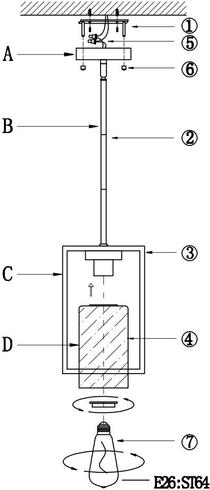
Installation sequence diagram
