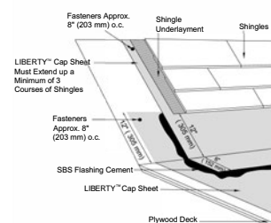
Shingle Tie-In
