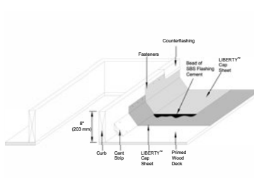
Wall-Curb Flashing
