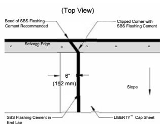
End Lap
