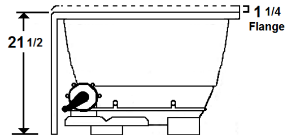
Standard (S) Silent Pump w/ Heater & Blower Location
