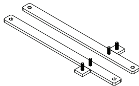
MOUNT BARS FOR CASTERS (2X)
