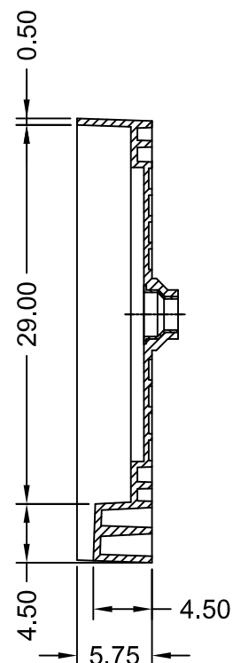
SECTION B-B
