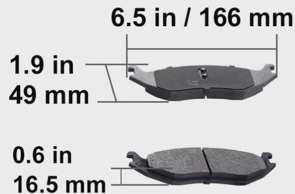
Brake pad Rear (P-967)
