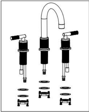
1.Loosen the nut of spout and handle;
