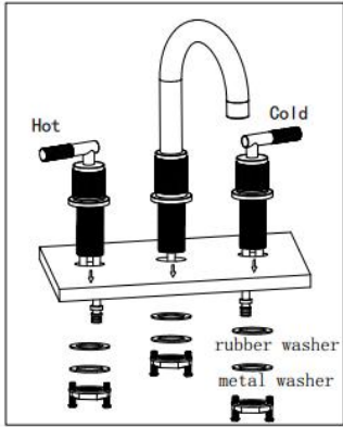
2.Place spout into the center hole of sink,place the handle body into right/left sink hole (Hot water handle in left,cold water handle right)Assemble rubber washer and metal washer then tighten the lock nut;
