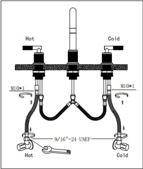
4.Connect two handles & two water supplies by water supply hose(Hot handle to Hot supply,Cold handle to Cold supply).
