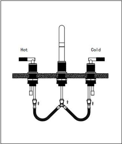
3.Connect the 2 handles and spout with quick connect hose;
