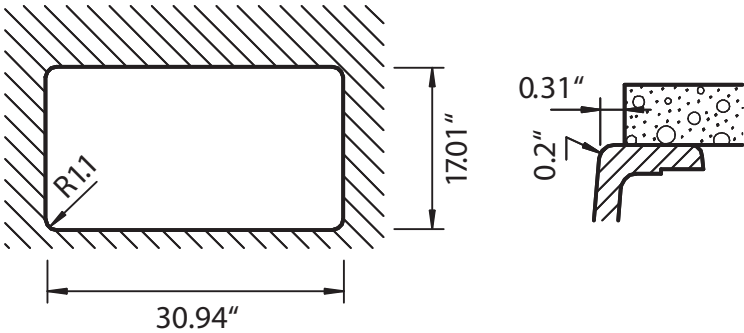
Installation: undermount cut-out
