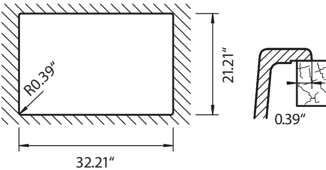
Installation: topmount cut-out
