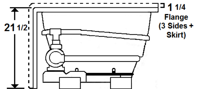
Standard (S) Pump, Blower, & Heater Location
