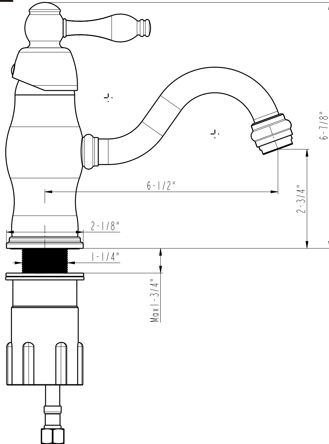
40118-Dimensional drawing
