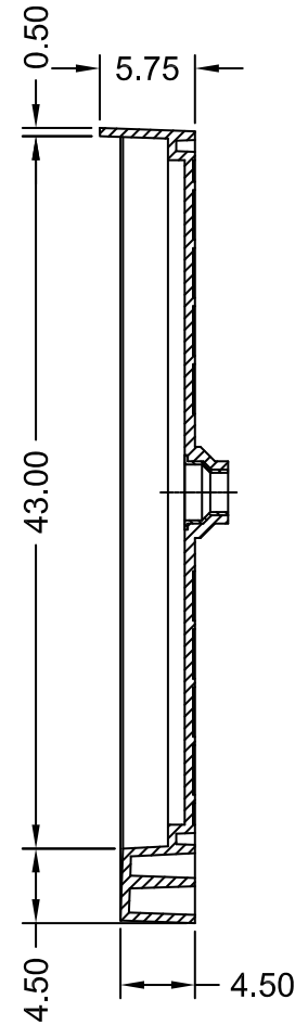
SECTION B-B
