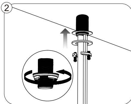
3-hole installation
