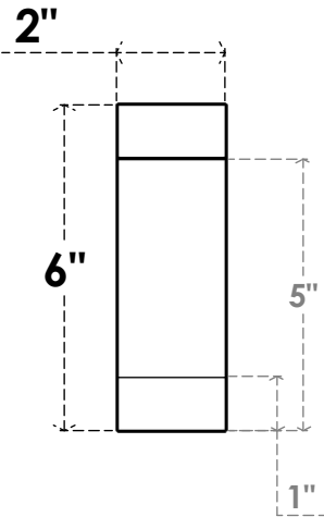
FRONT PROFILE
