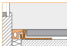
4.9 Schluter®-DILEX-KSA
