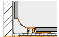
4.15 Schluter®-DILEX-HKS
