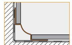
4.15 Schluter®-DILEX-EHK
