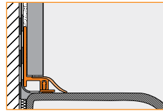
4.10 Schluter®-DILEX-AS
