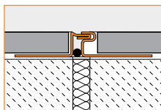
4.16 Schluter®-DILEX-EDP
