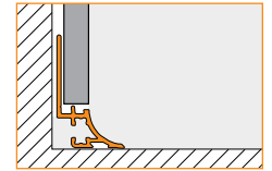
4.22 Schluter®-DILEX-AHKA
