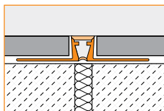
4.6 Schluter®-DILEX-BWB
