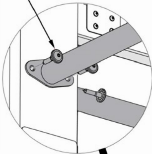
471 (x8) LAG SCREW - 1 1/2"
