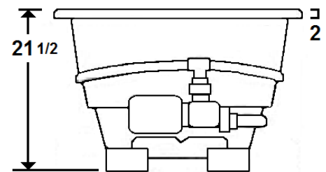
Standard (S) Silent Pump w/ Heater Location
