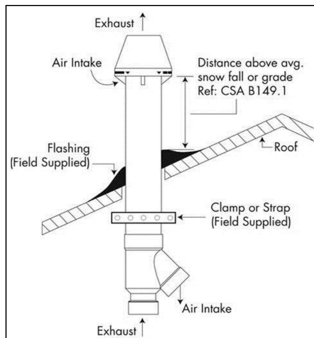
Roof Termination
