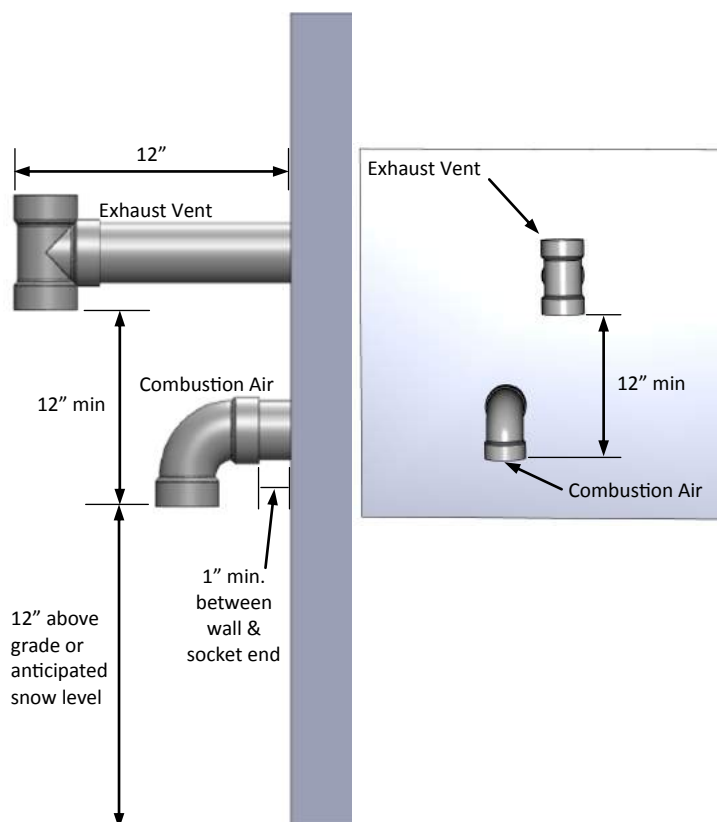
Sidewall Vent and Combustion Air Piping with Tee Termination
