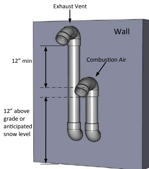
Sidewall Vent and Combustion Air Piping with Snorkel Termination
