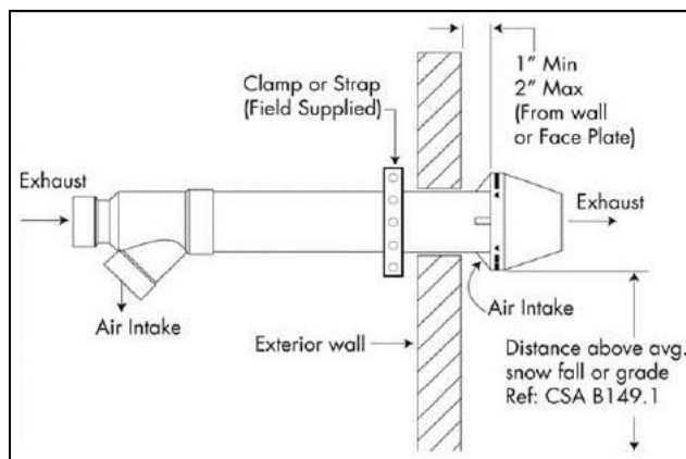
Wall Termination
