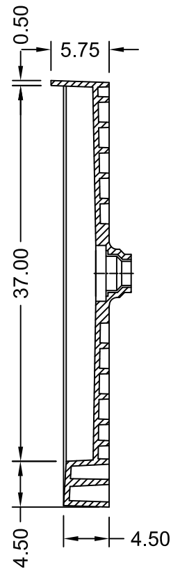
SECTION B-B
