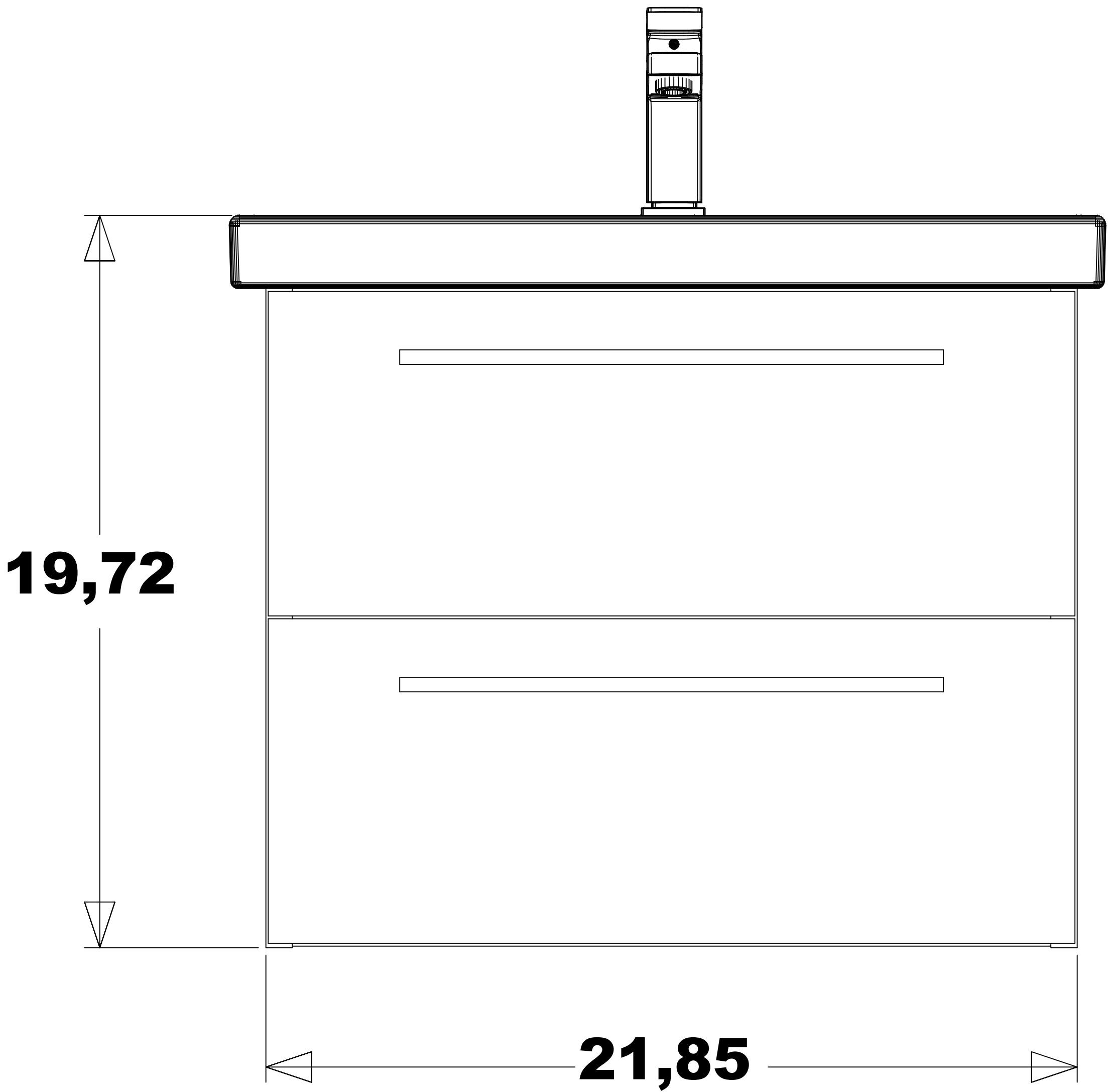
FRONT VIEW
