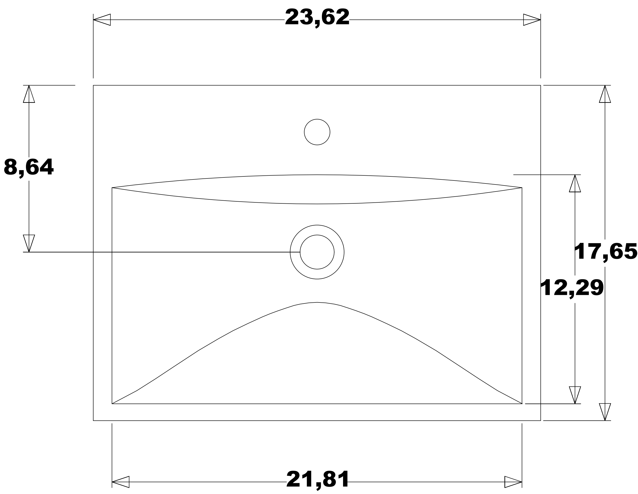
TOP VIEW
