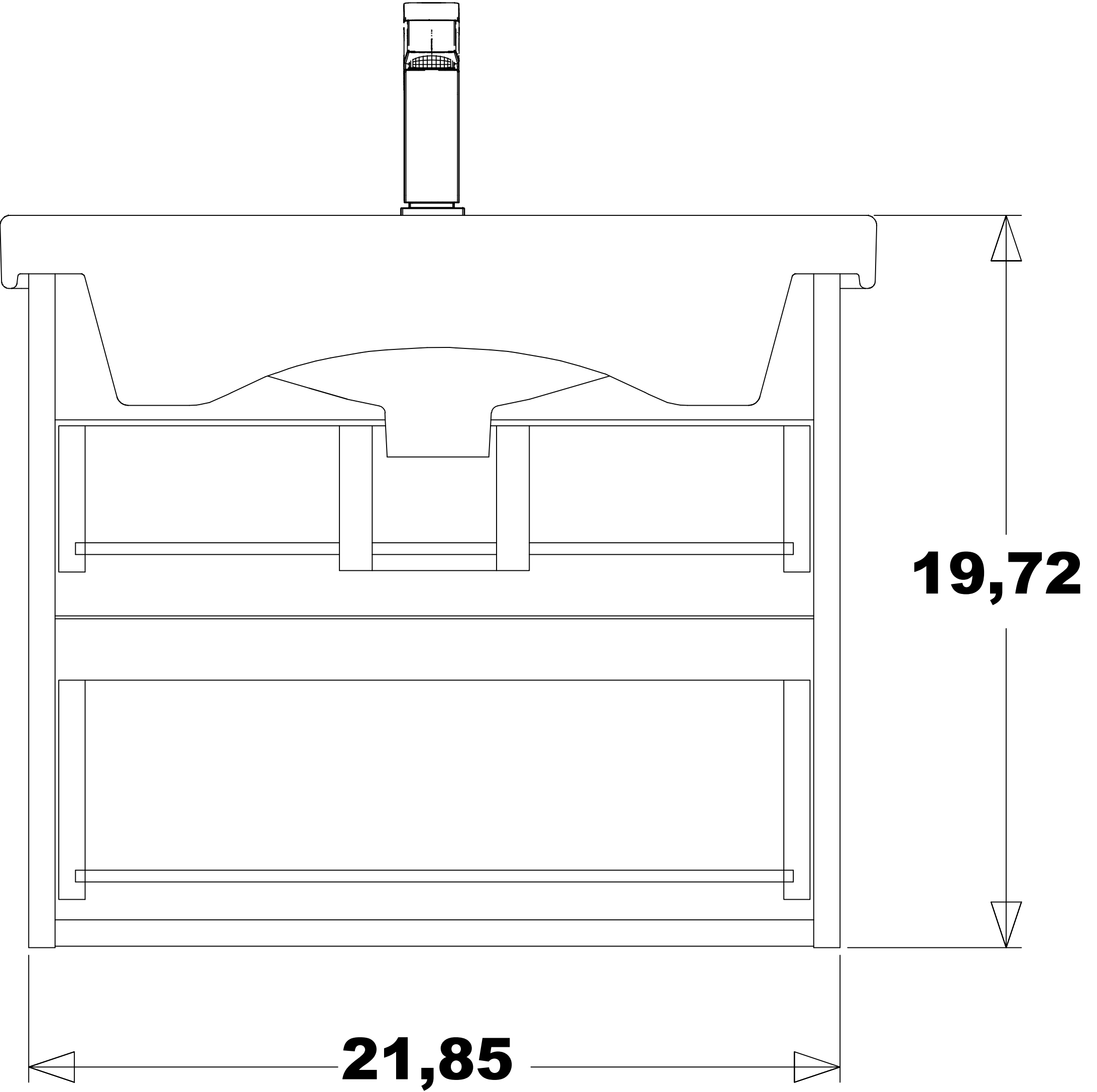
BACK VIEW
