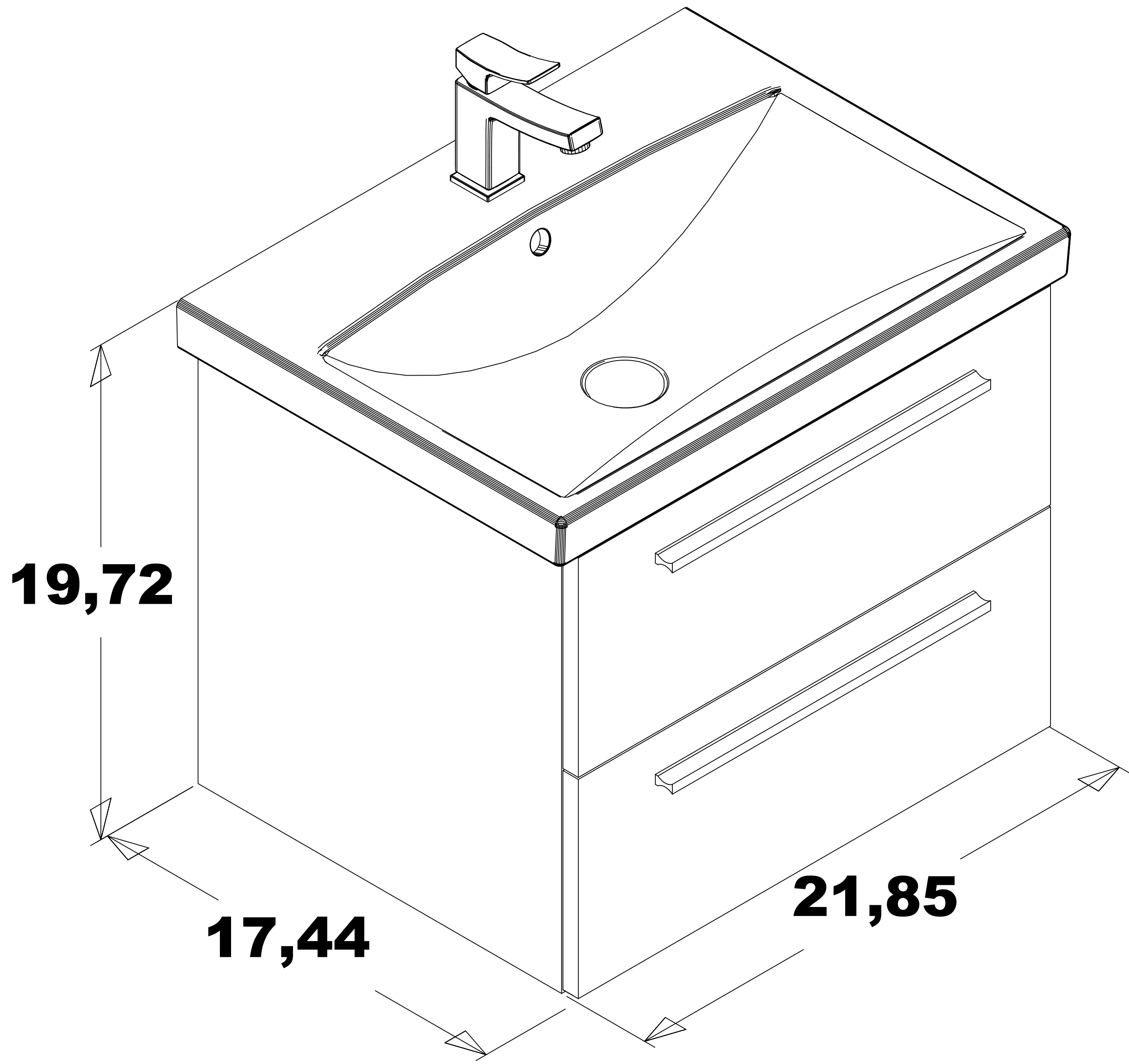
ISOMETRIC VIEW
