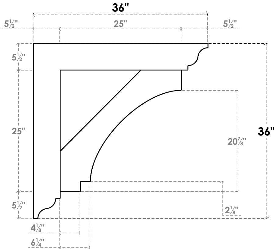
SIDE PROFILE
