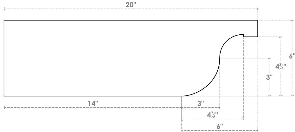
SIDE PROFILE
