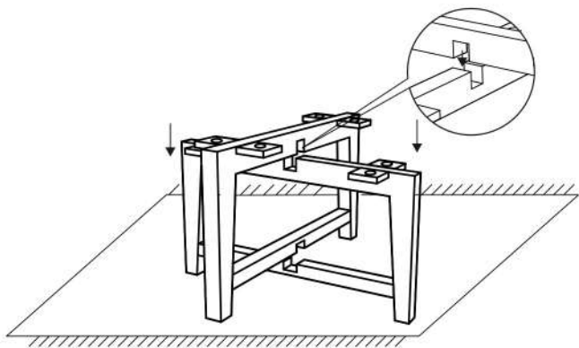
Step 1: Insert the legs in each other to make complete base
