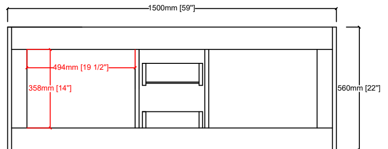
BACK VIEW
