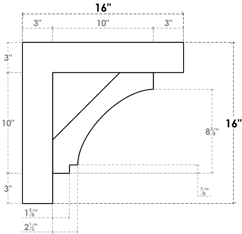
SIDE PROFILE
