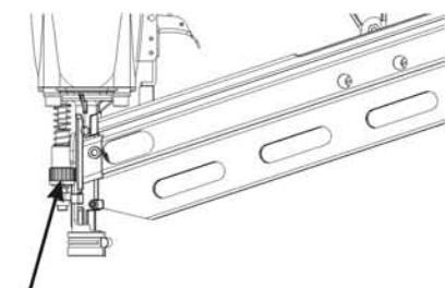
Adjustment wheel(C)
