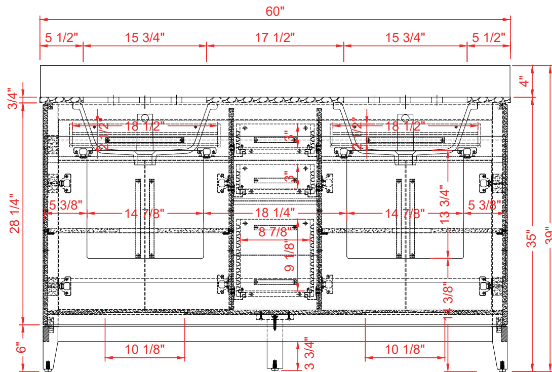
FRONT VIEW
