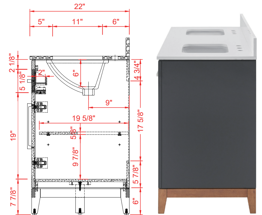
SIDE VIEW
