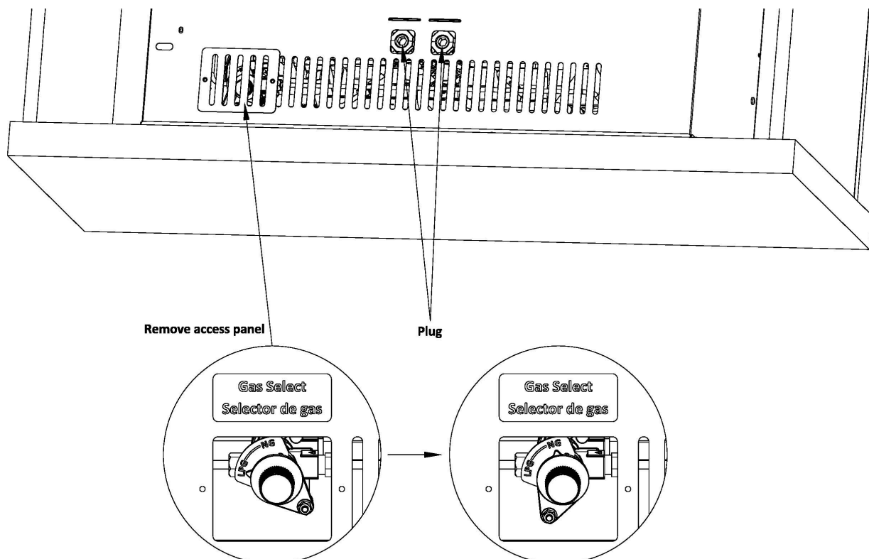
Fig. 12—Gas Selection
