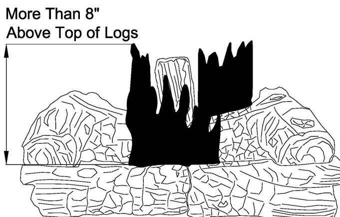
Fig. 25—Incorrect Burner Flame Pattern
