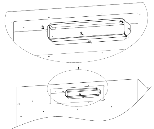
Fig. 7—Attaching Thermal Switch Bracket
