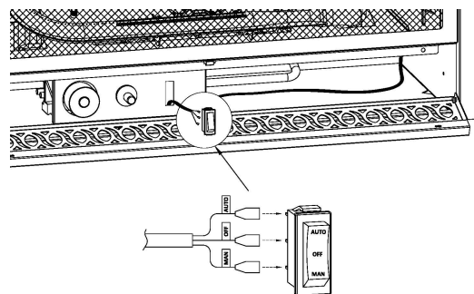
Fig. 9—Connecting Switch
