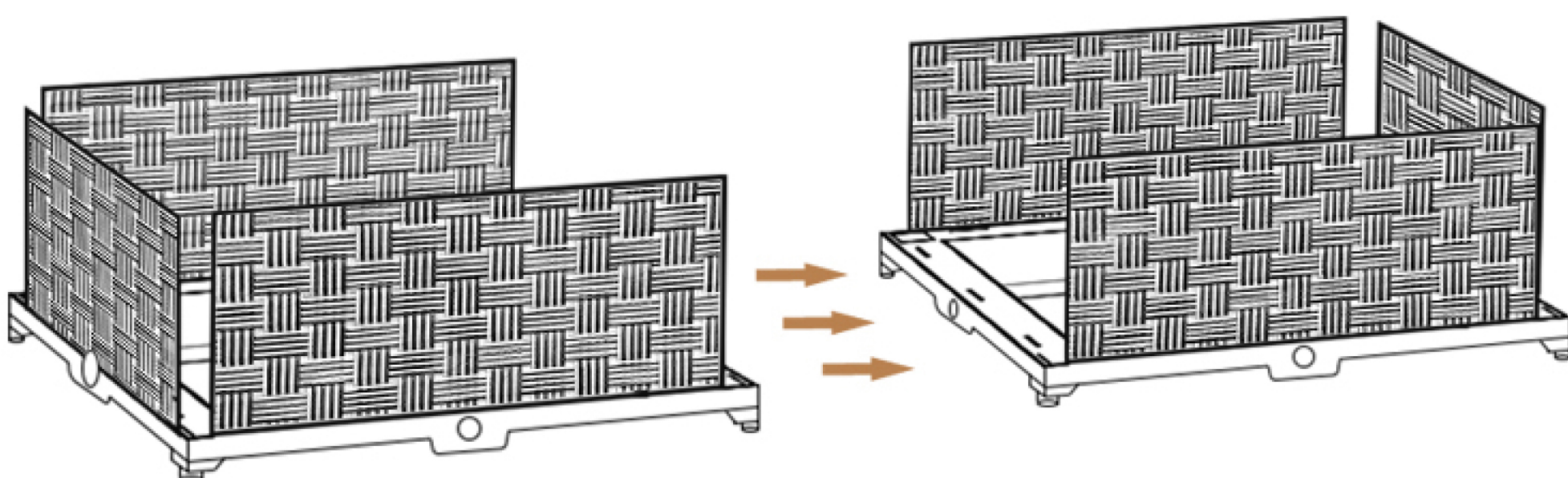
Step 3: Connect the two spliced parts.
