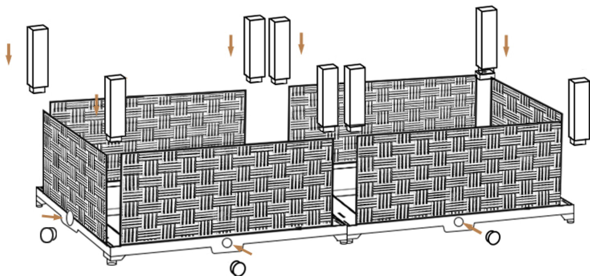
Step 4: Insert the connecting rod into the slot
